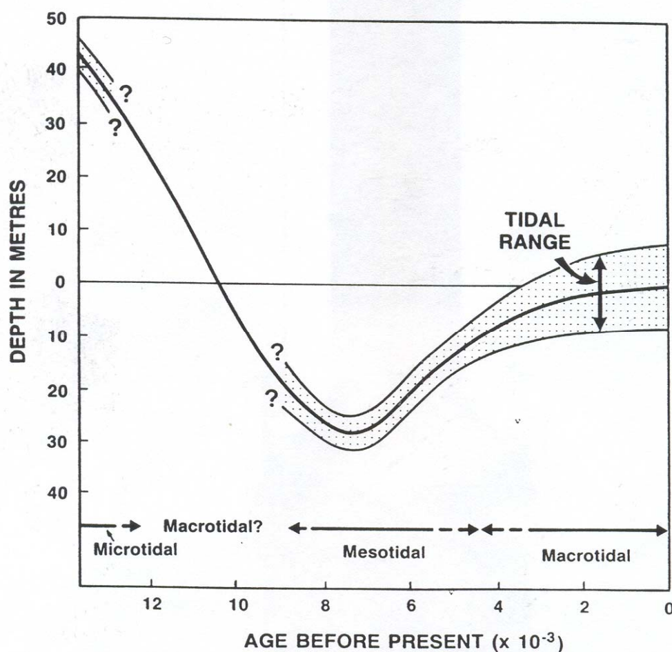
Figure 3b. History of sea level and tidal range in the inner Bay of Fundy, based on data from Chignecto Bay (after Amos and Zaitlin, 1985). A similar pattern of sea-level and tidal range oscillations have occurred in the Minas Basin but with smaller amplitudes.
