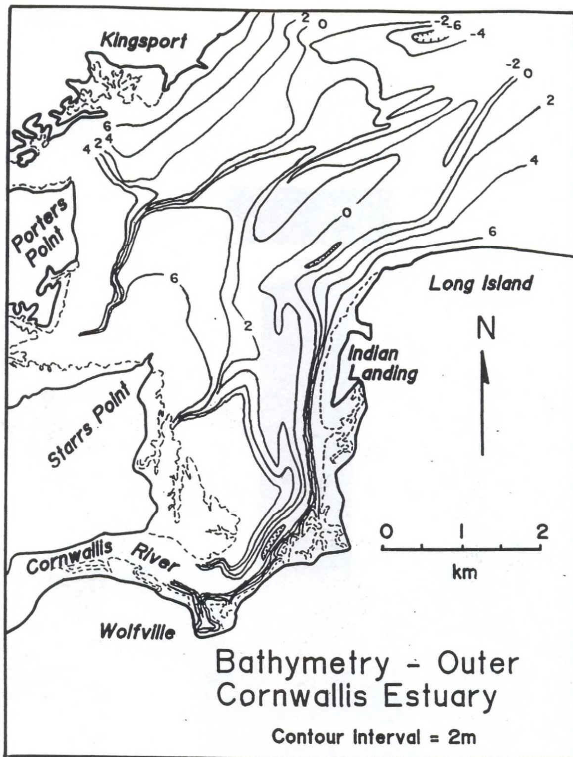
Figure 4. Bathymetry of the outer Cornwallis River. Datum is approximately mean low water. Note the development of flood "barbs" along the west side of the Cornwallis River channel.
