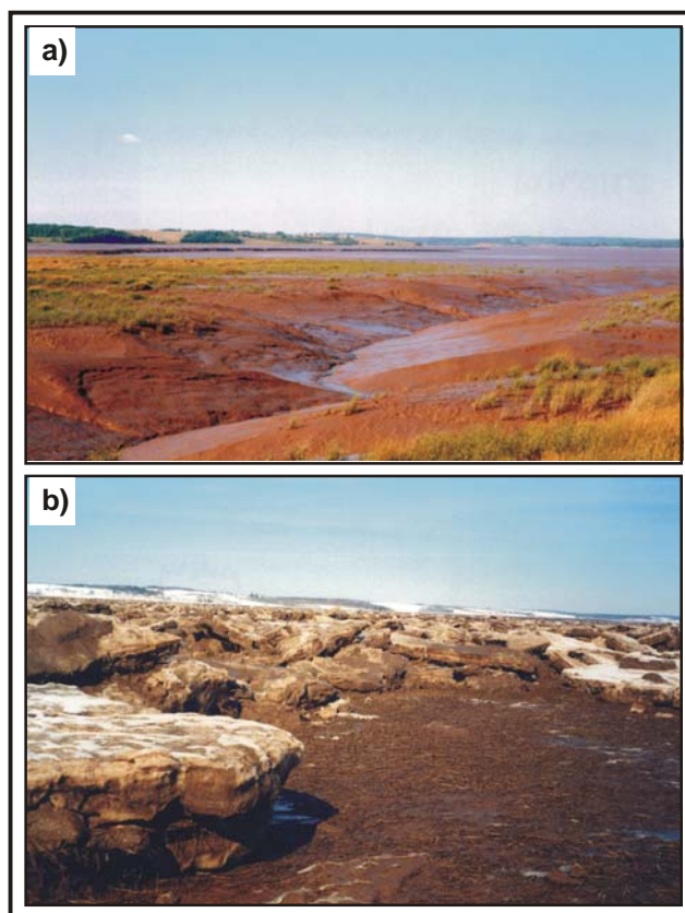
Figure 8. a) Windsor salt marsh in late Fall, 2002; b) same location in February, 2003.
