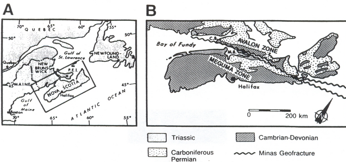
Figure 3a. A: Location map of eastern Canada. B: Geological and location map of the Bay of Fundy region. M.B. Minas Basin; C.B. Chignecto Bay.
