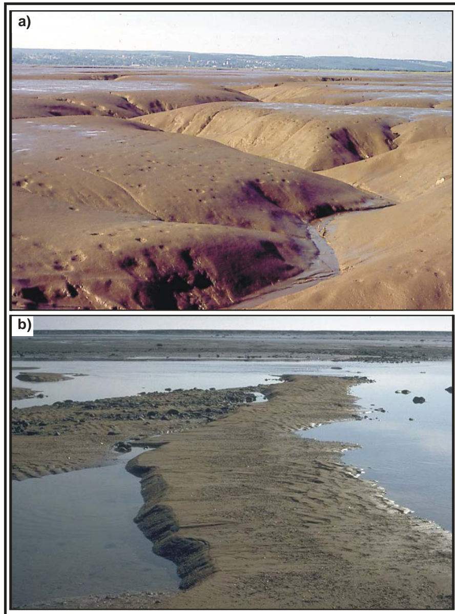
Figure 13. a) Mudflats and channels of the inner Southern Bight (Starr's Point); b) Dune with superimposed ripples in the Southern Bight, (near Evangeline Beach)
