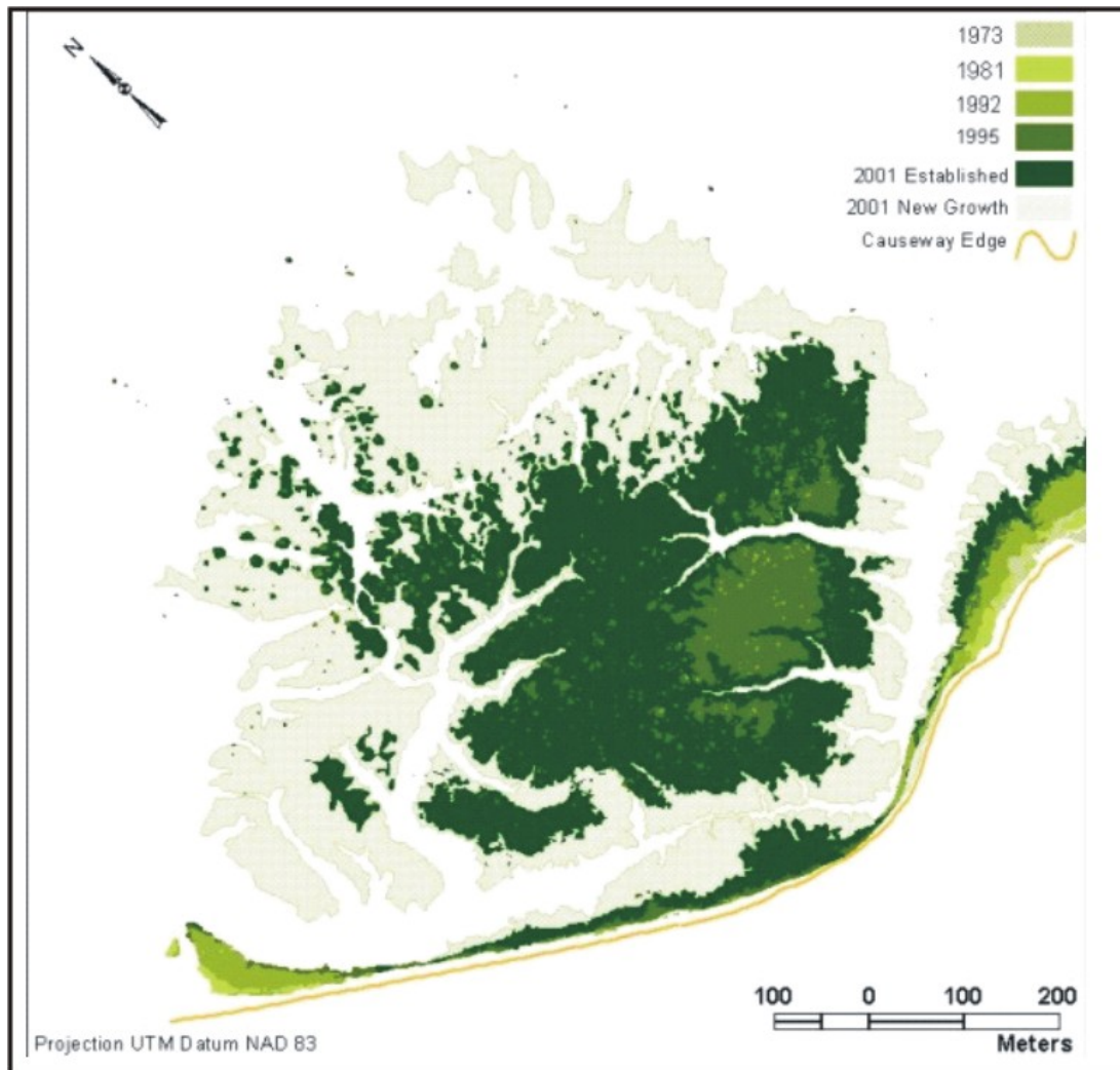
Figure 10: GIS analysis of spatial patterns of colonization by S. alterniflora in 1973, 1981, 1992, 1995 and juvenile and mature or established S. alterniflora surveyed in 2001 (van Proosdij and Townsend, 2004a).
