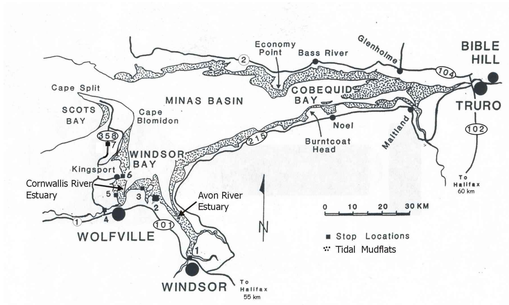
Figure 2. Map of the Minas Basin-Cobequid Bay-Salmon River area showing the location of the stops to be visited on the map.
