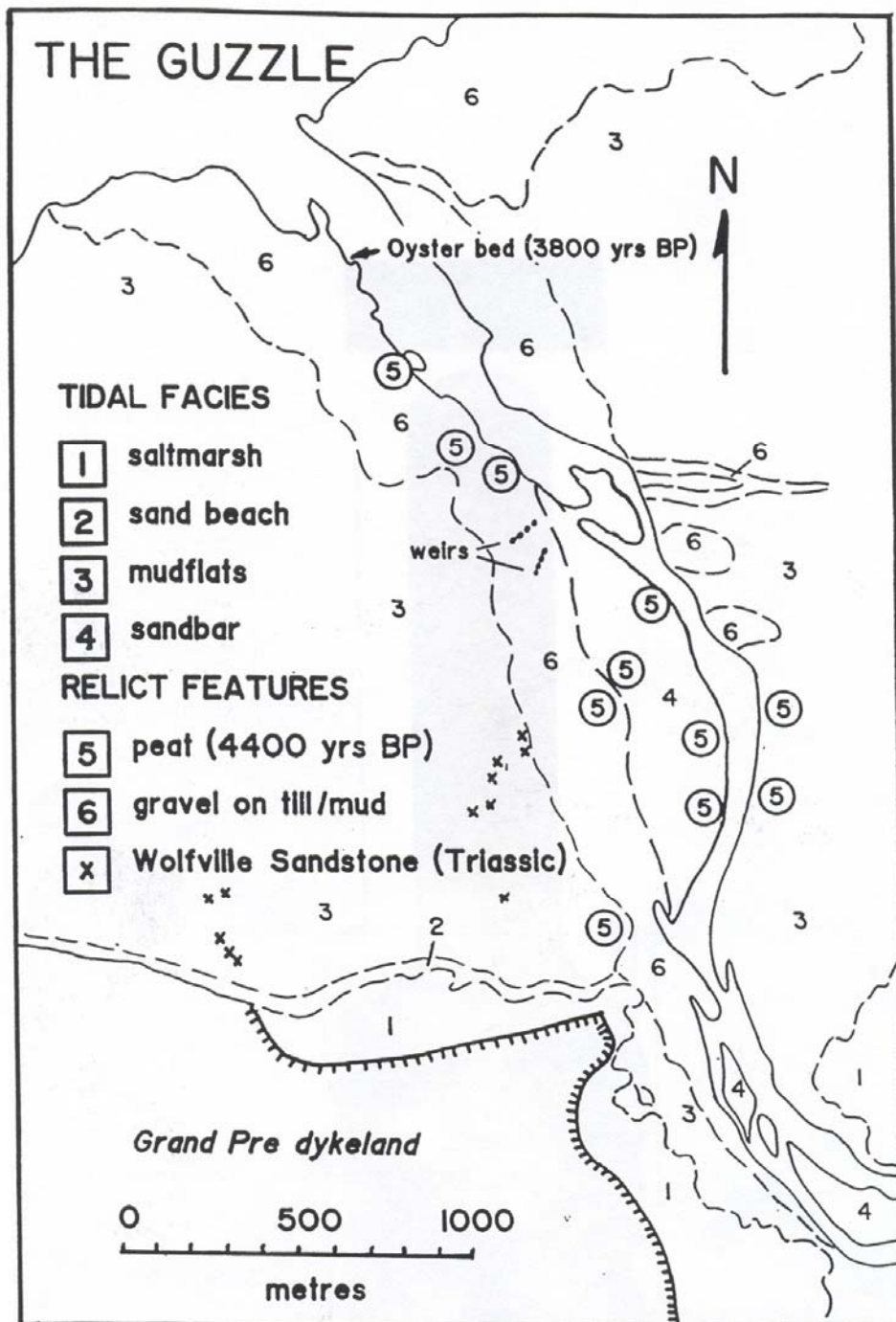
Figure 12. Sketch map of The Guzzle area at Evangeline Beach showing the distribution of major facies and features.
