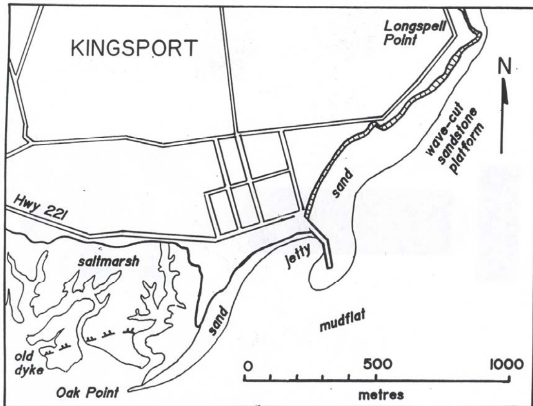
Figure 18. Sketch map of Kingsport at the seaward limit of the Cornwallis estuary. Saltmarsh and Mudflats of the outer estuary give way between Oak Point and Kingsport wharf to a sediment-starved, wave-cut platform with a sand beach at the high tide level. This change reflects a seaward increase in the influence of wave action, and a change from tide dominated to mixed energy sedimentation
