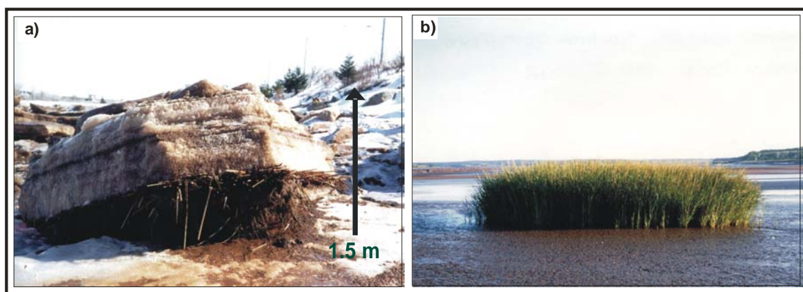
Figure 9. a) Ice cake containing sediment and rhizome material adjacent to the causeway in February 2002 and b) newly established ‘satellite’ of vegetation in July 2002 (van Proosdij and Townsend, 2004a).
