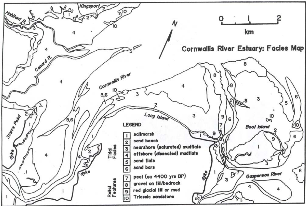
Figure 5. Facies distribution in the outer Cornwallis River estuary. Note the sandy facies are very restricted in extent, while fringing mudflats facies are extensive.
