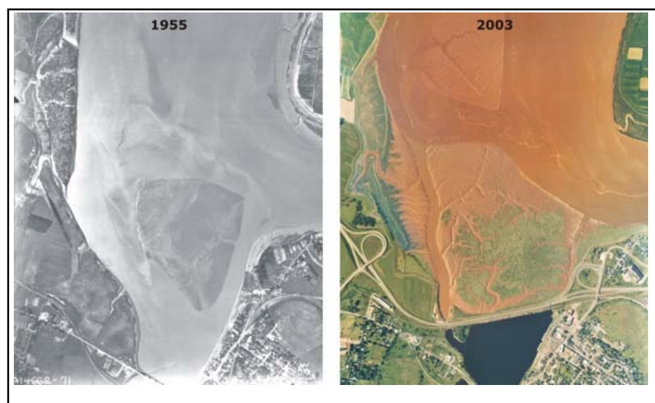
Figure 7. a) Avon River and Town of Windsor in 1955 at high tide before causeway construction and in b) 2003, after causeway construction and significant amounts of sediment had accumulated seaward of the barrier. Note the establishment of marsh vegetation.
