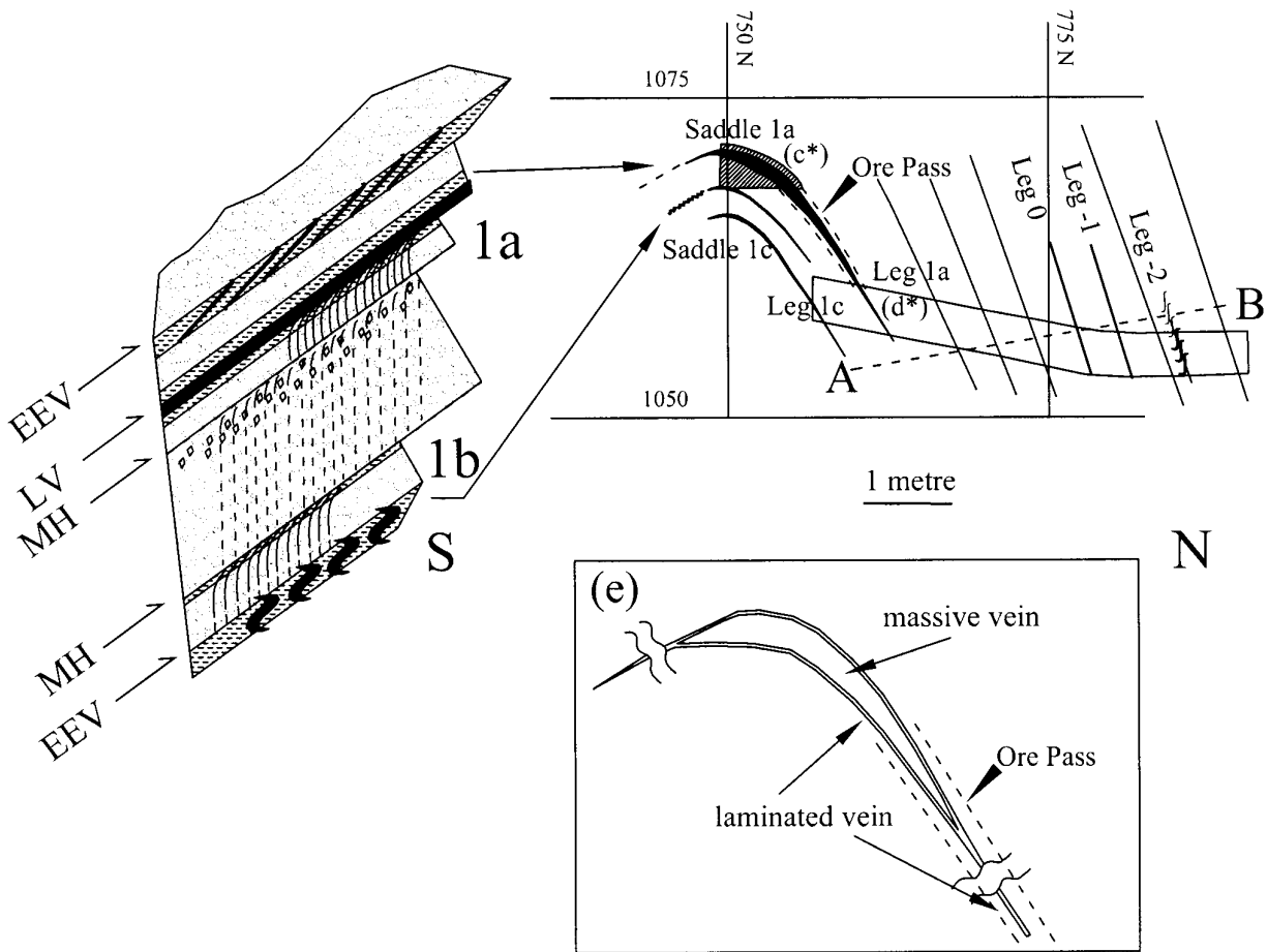
Figure 21: Cross section of Saddle 1 and structurally higher section of the north limb exposed in the decline. Detailed section at left shows detail of the stratigraphy and bedding-concordant movement horizons and en echelon veins associated with the south limb of the saddle as exposed in the 1066 stope. Lower figure, labeled (e), shows the geometry of the saddle and the distribution of laminated vein at the margin of the saddle.
