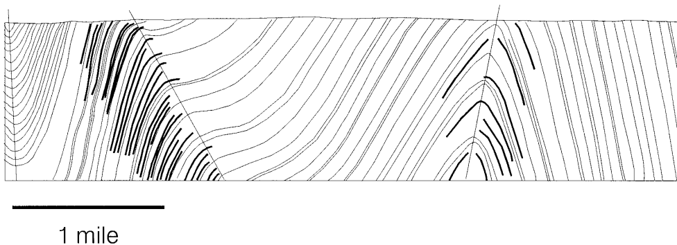
Figure 4c: Cross section showing the distribution of the Waverley and Montague gold districts on the north and south limbs of an anticlinorium (see cross section in Fig 1 for reference). Bedding-concordant veins at each district occur primarily on the steep limbs, which represent the limbs of the anticlinorium.
